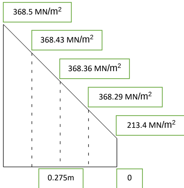
Figure 33 Shear Force Diagram
