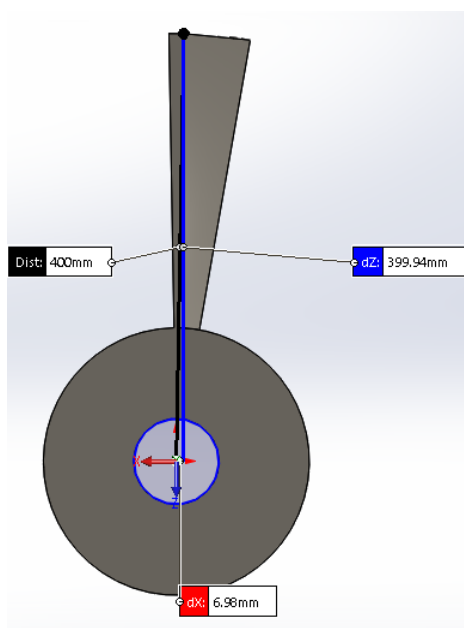
Figure 13 Single Turbine Blade Design
