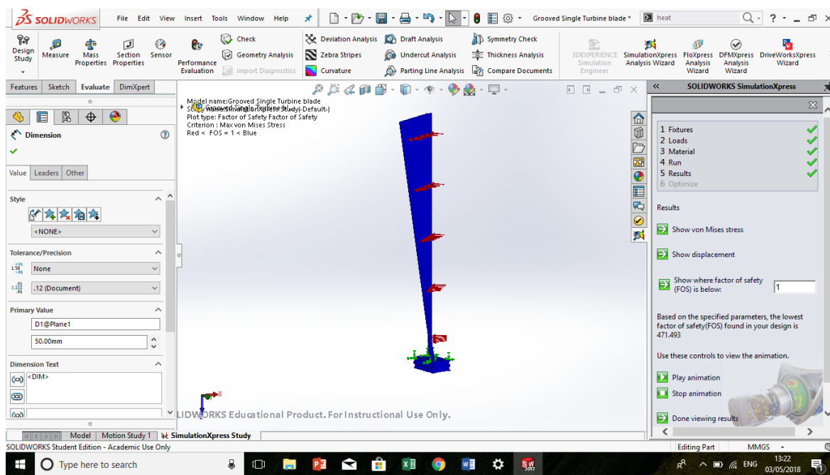
Figure 26 Safety Factor
